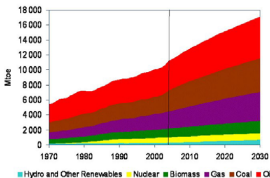
World Primary Energy Demand by Fuel in the Reference Scenario
